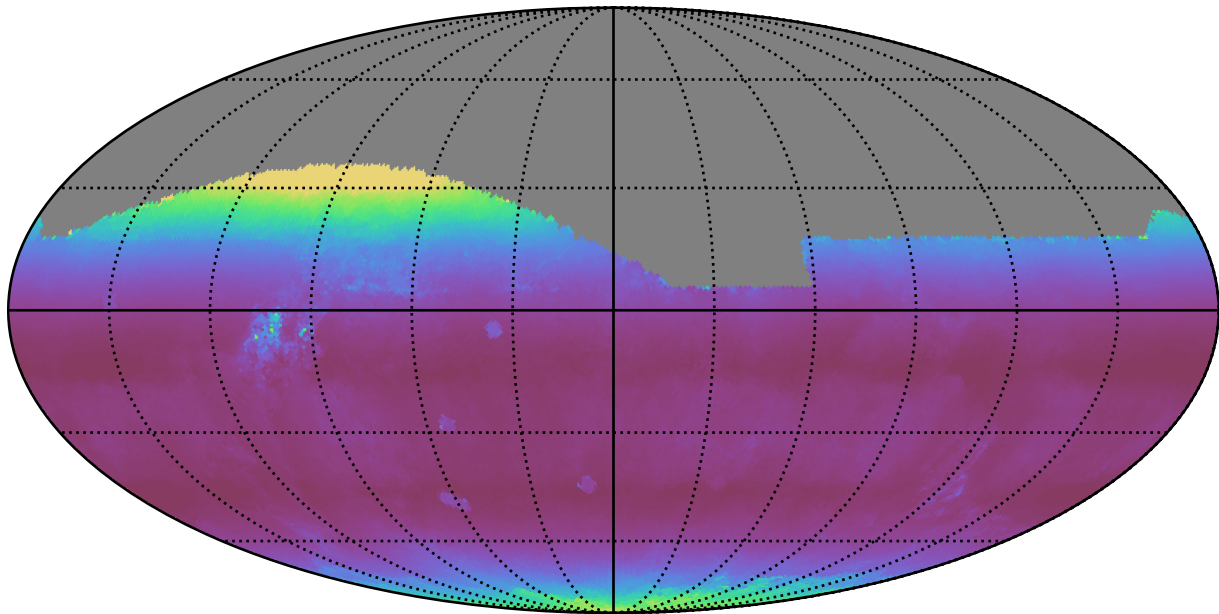
too_elab_r16_d2_gz_v3.4_10yrs All sky r band: Median airmass
