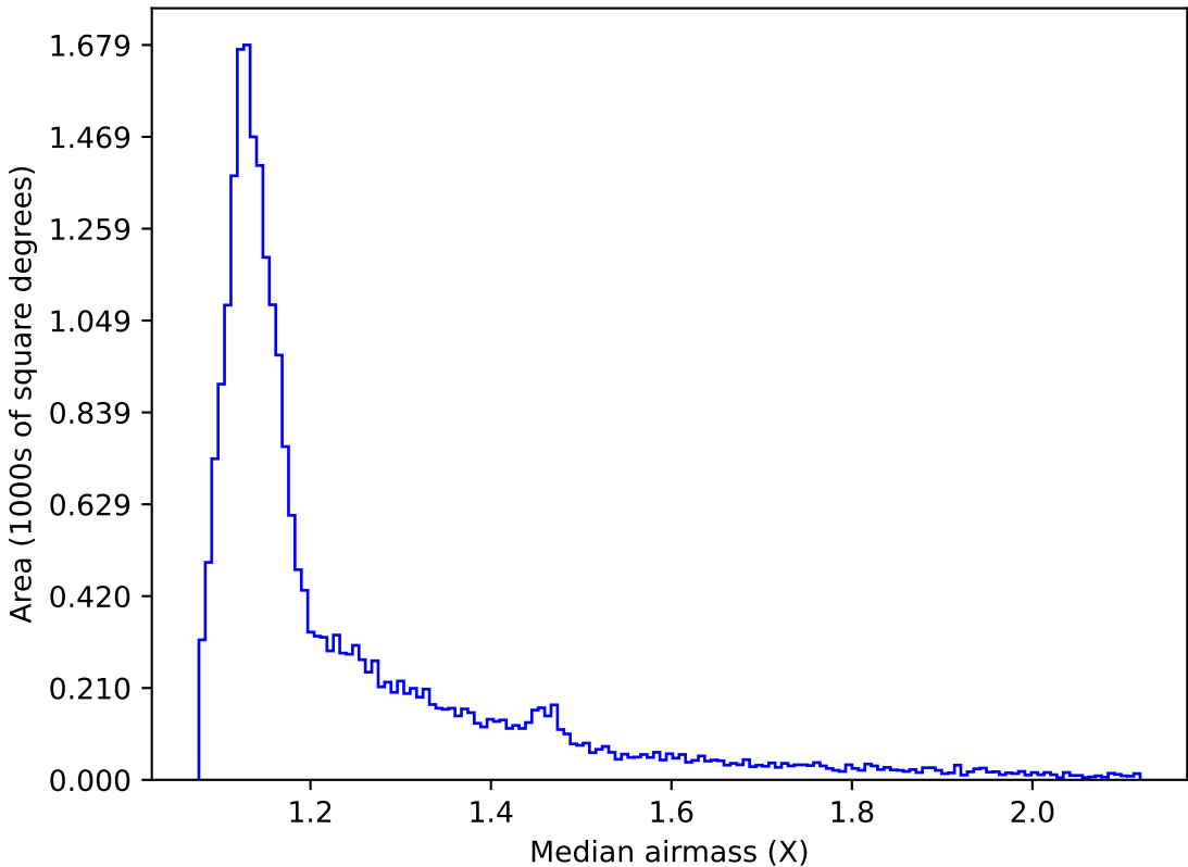
too_elab_r16_d2_gz_v3.4_10yrs All sky r band: Median airmass
