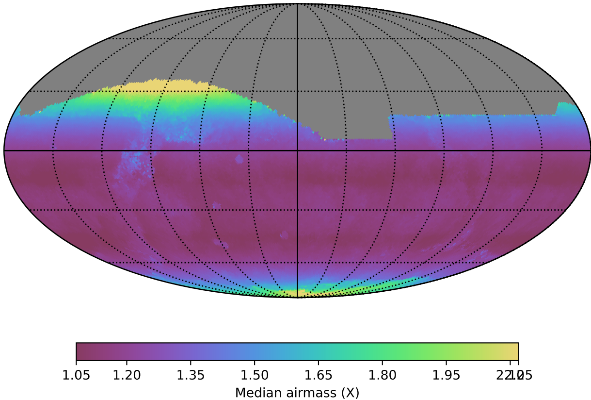
too_elab_r16_d2_gz_v3.4_10yrs All sky i band: Median airmass
