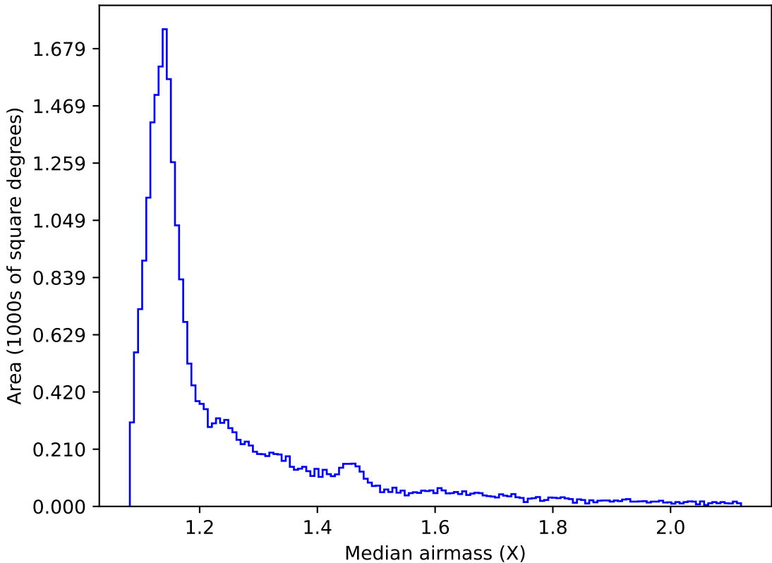
too_elab_r16_d2_gz_v3.4_10yrs All sky i band: Median airmass
