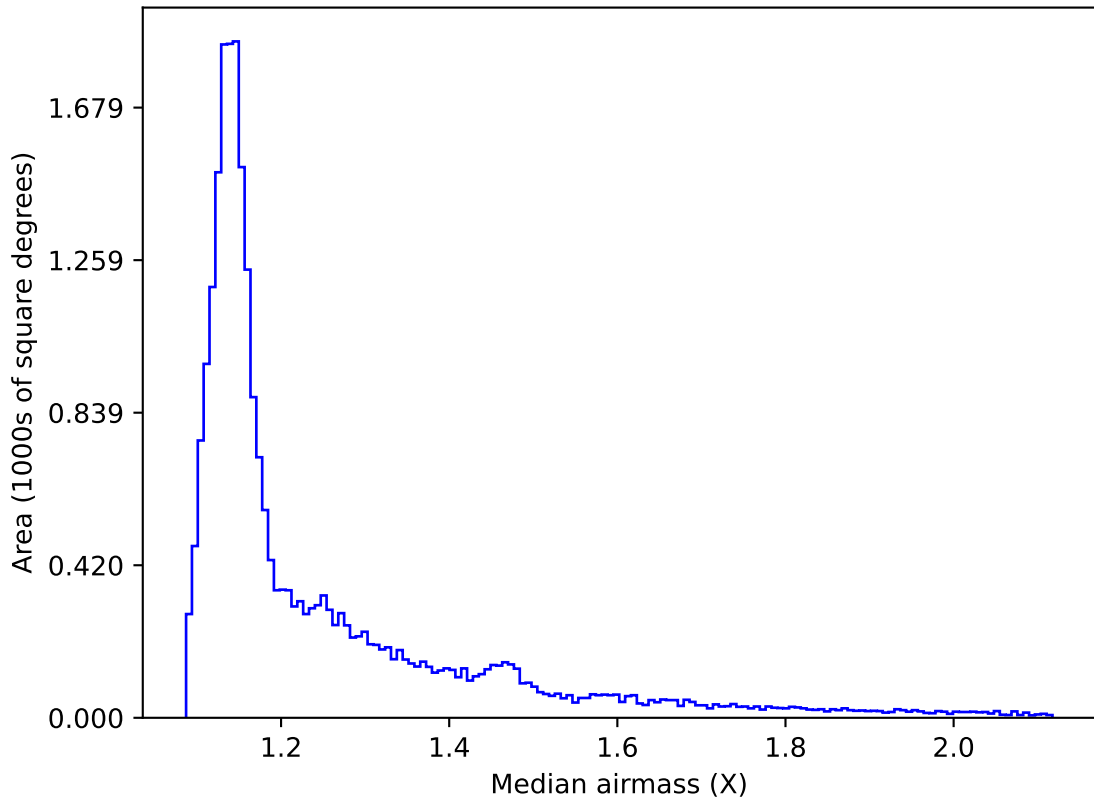
too_elab_r16_d2_gz_v3.4_10yrs All sky all bands: Median airmass
