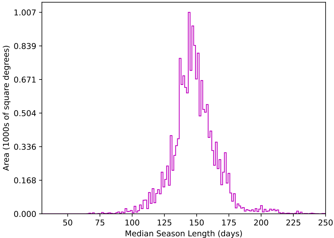
too_elab_r16_d2_gz_v3.4_10yrs WFD z band: Median Season Length
