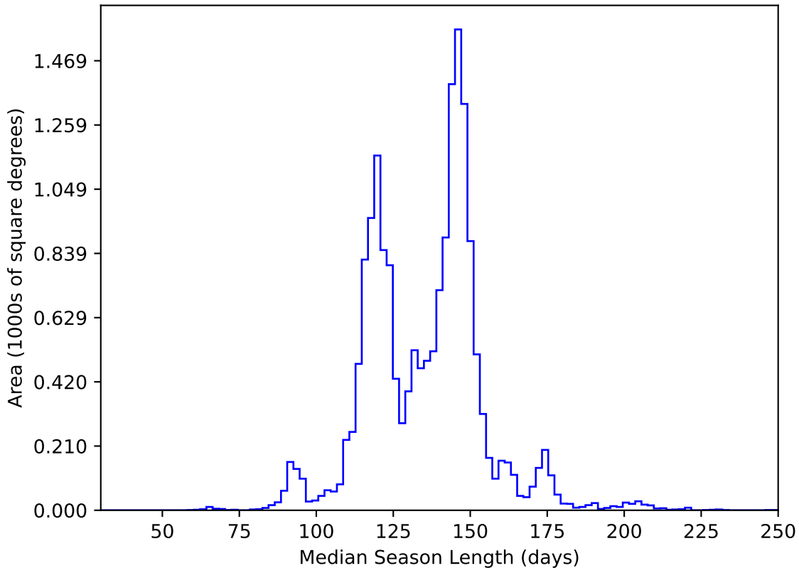
too_elab_r16_d2_gz_v3.4_10yrs WFD y band: Median Season Length
