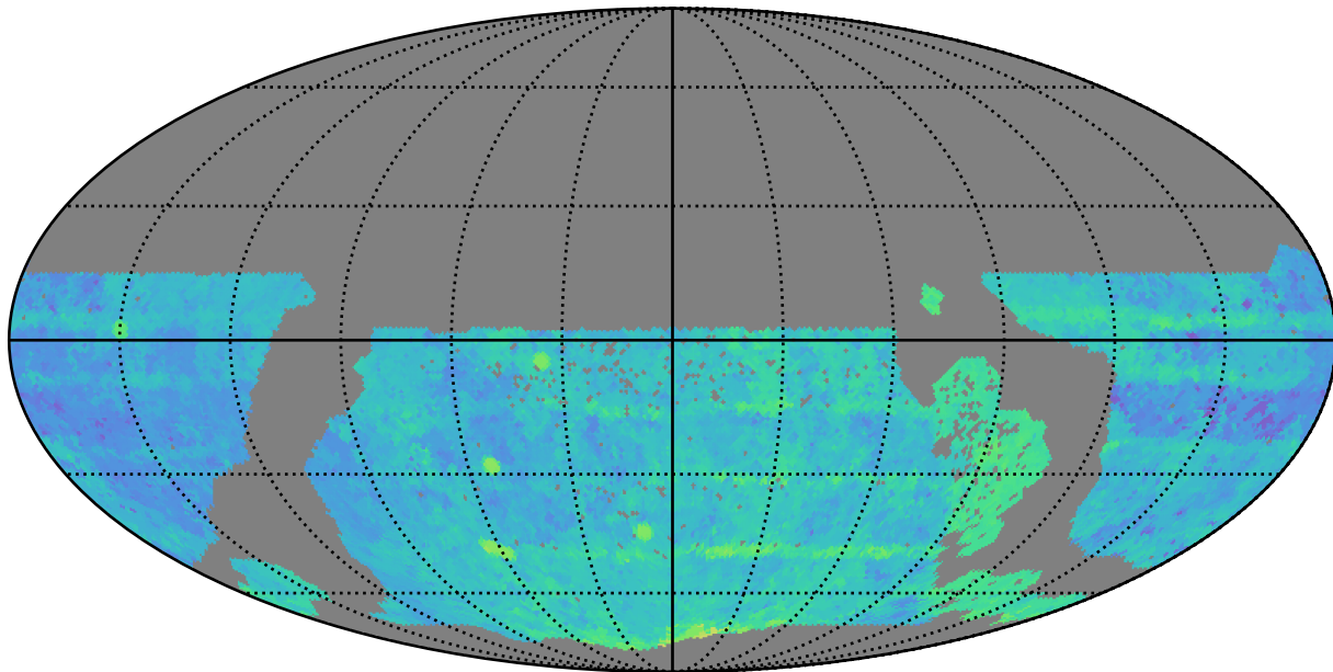
too_elab_r16_d2_gz_v3.4_10yrs WFD r band: Median Season Length
