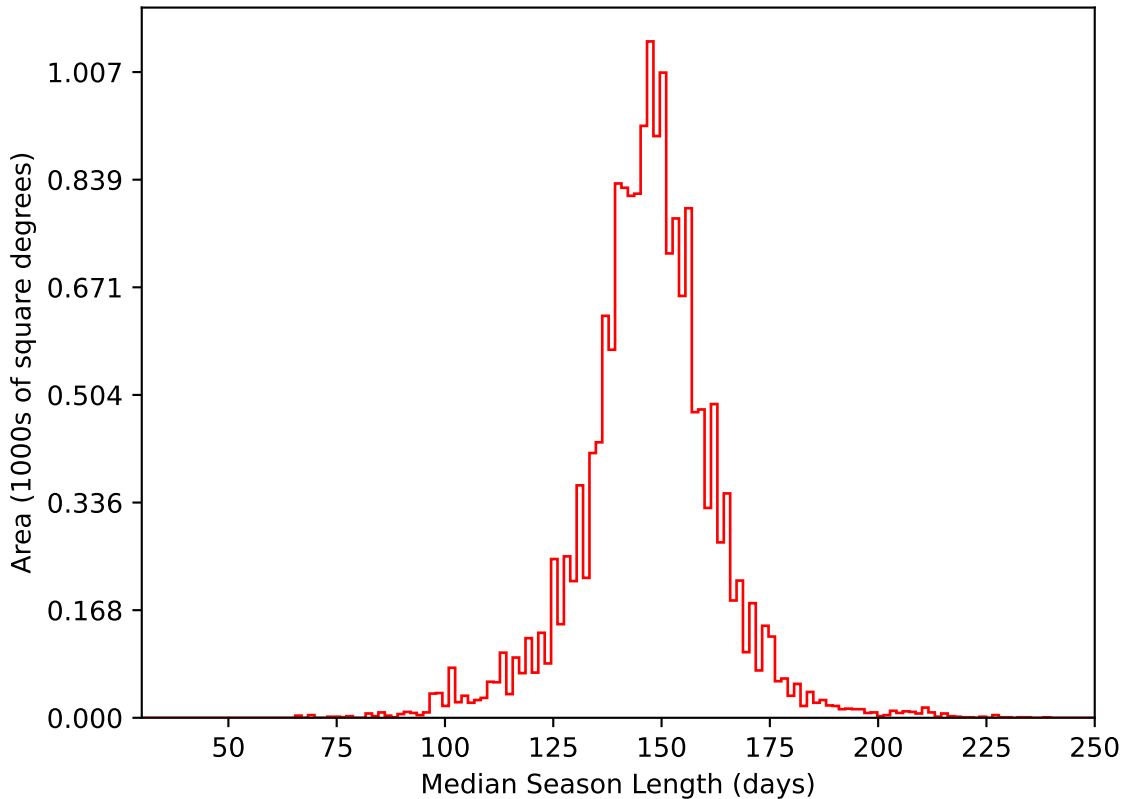
too_elab_r16_d2_gz_v3.4_10yrs WFD i band: Median Season Length
