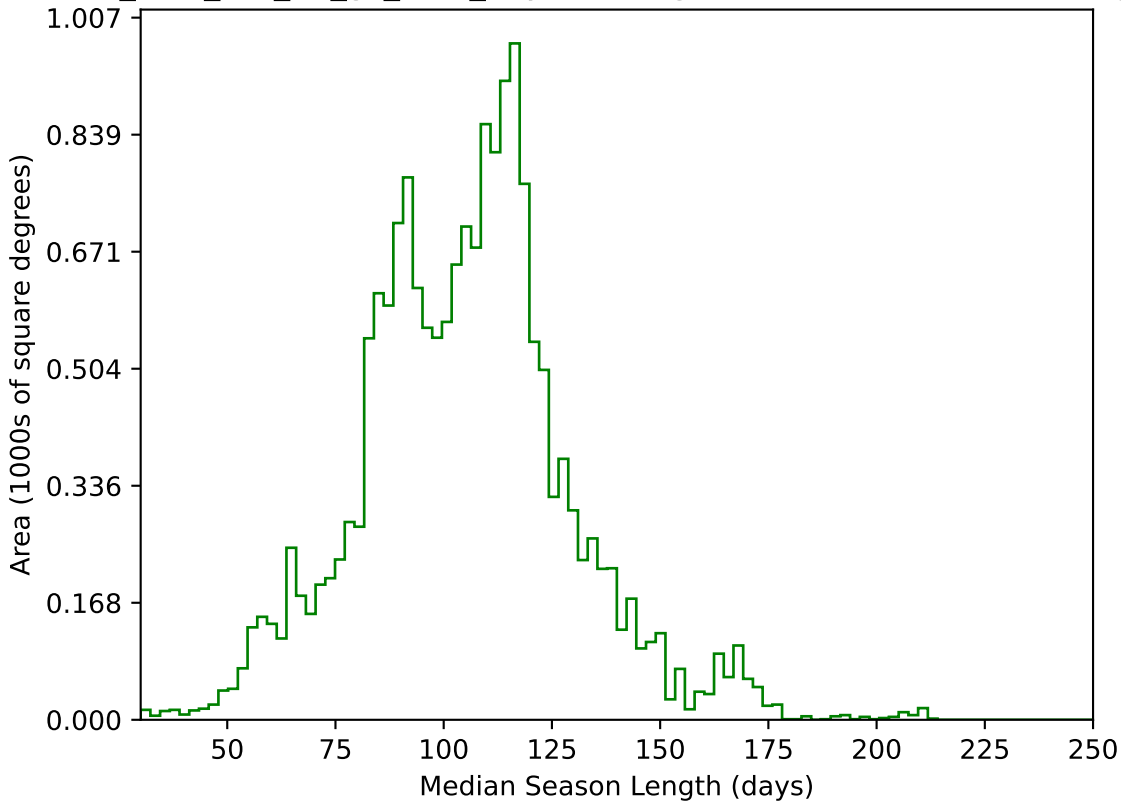
too_elab_r16_d2_gz_v3.4_10yrs WFD g band: Median Season Length
