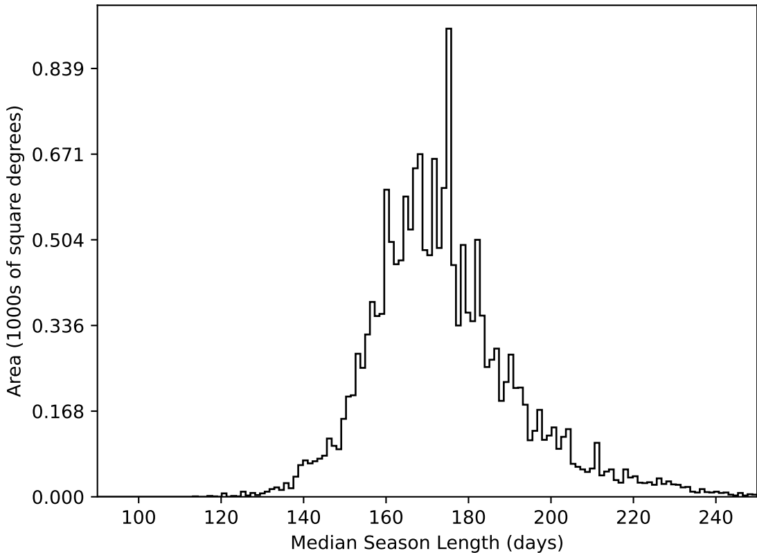
too_elab_r16_d2_gz_v3.4_10yrs WFD all bands: Median Season Length
