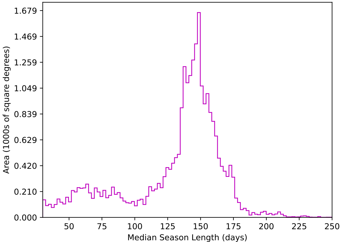
too_elab_r16_d2_gz_v3.4_10yrs All sky z band: Median Season Length
