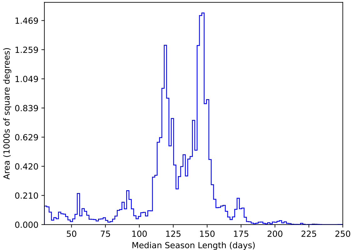
too_elab_r16_d2_gz_v3.4_10yrs All sky y band: Median Season Length
