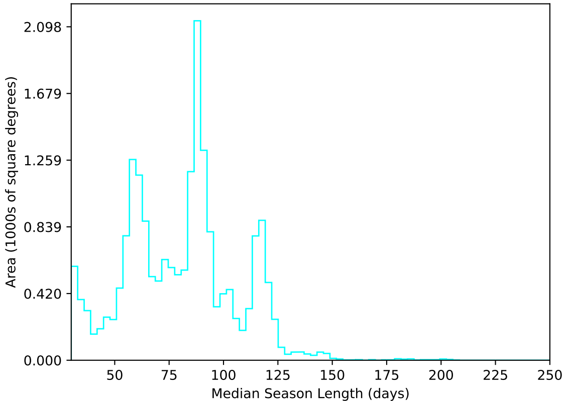
too_elab_r16_d2_gz_v3.4_10yrs All sky u band: Median Season Length
