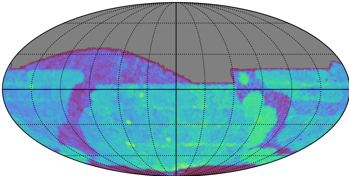
too_elab_r16_d2_gz_v3.4_10yrs All sky r band: Median Season Length
