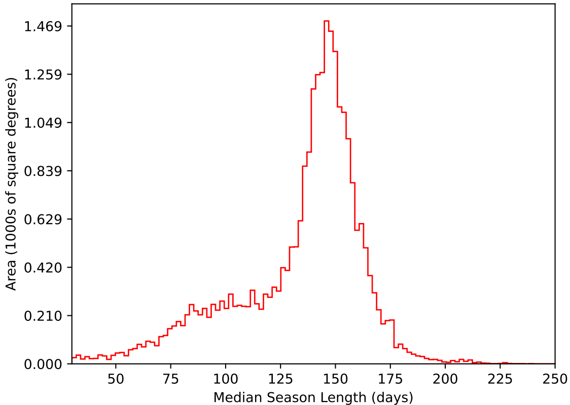
too_elab_r16_d2_gz_v3.4_10yrs All sky i band: Median Season Length
