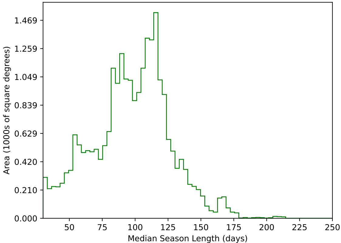
too_elab_r16_d2_gz_v3.4_10yrs All sky g band: Median Season Length
