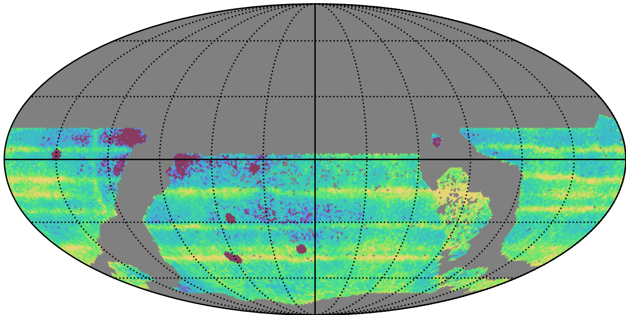
too_elab_r16_d2_gz_v3.4_10yrs WFD: Median Intra-Night Gap
