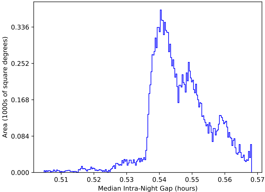
too_elab_r16_d2_gz_v3.4_10yrs WFD: Median Intra-Night Gap
