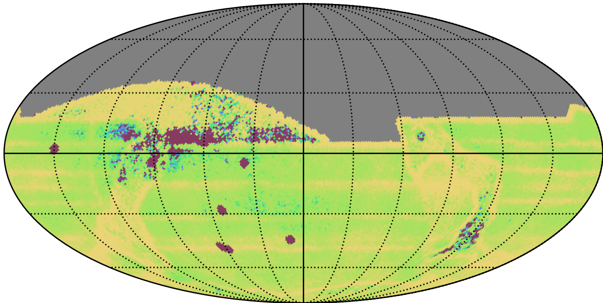
too_elab_r16_d2_gz_v3.4_10yrs All sky: Median Intra-Night Gap
