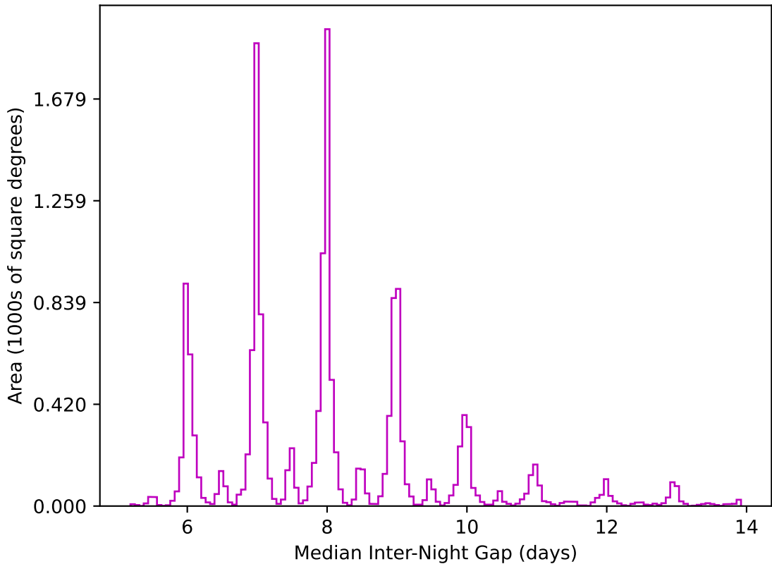
too_elab_r16_d2_gz_v3.4_10yrs WFD z band: Median Inter-Night Gap
