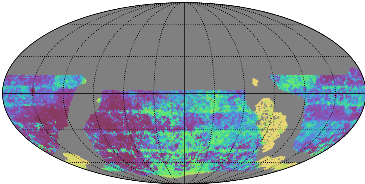
too_elab_r16_d2_gz_v3.4_10yrs WFD y band: Median Inter-Night Gap
