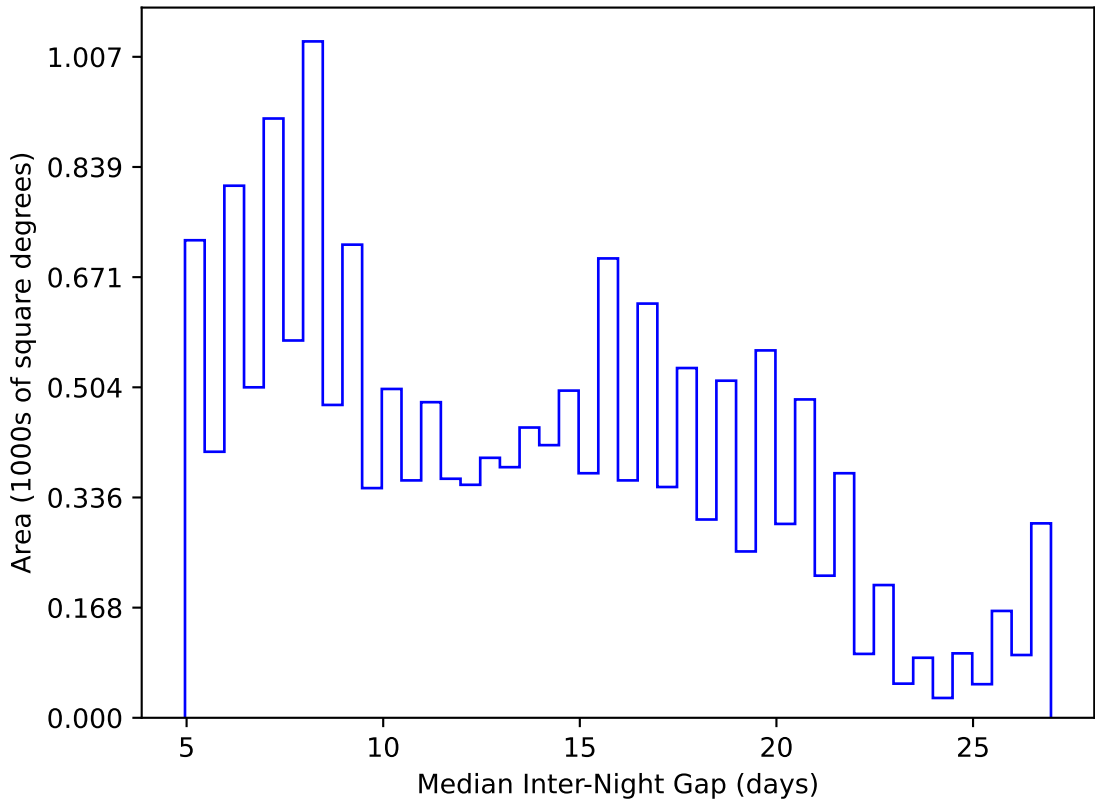
too_elab_r16_d2_gz_v3.4_10yrs WFD y band: Median Inter-Night Gap
