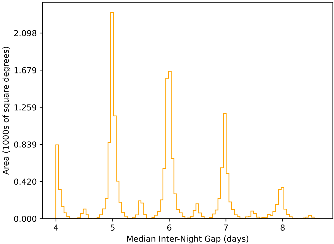
too_elab_r16_d2_gz_v3.4_10yrs WFD r band: Median Inter-Night Gap
