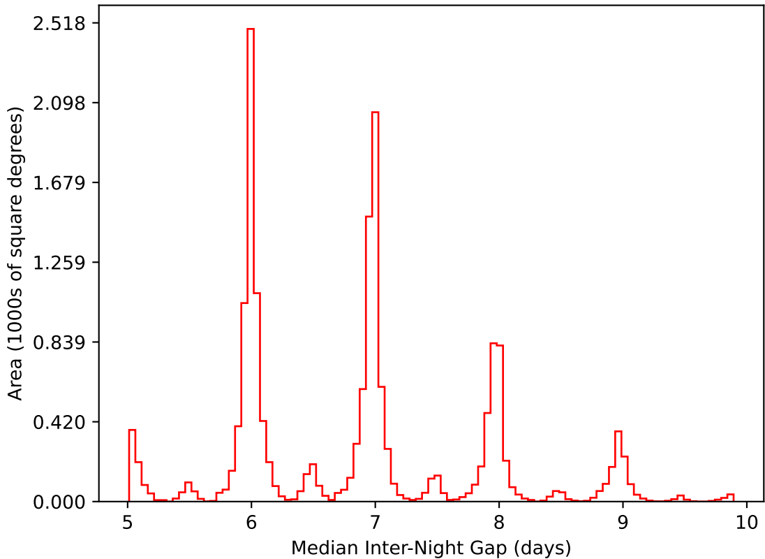
too_elab_r16_d2_gz_v3.4_10yrs WFD i band: Median Inter-Night Gap
