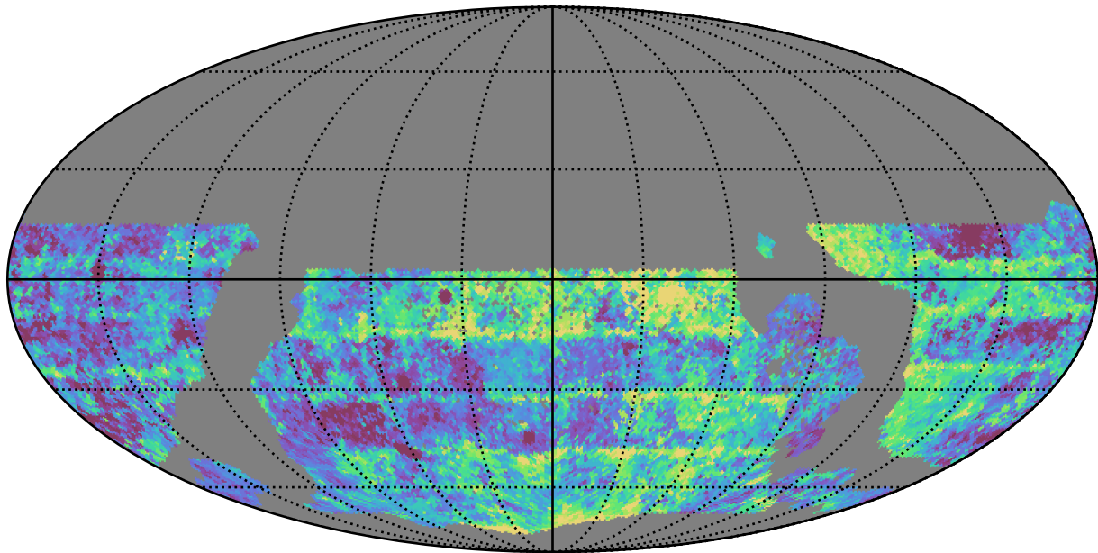
too_elab_r16_d2_gz_v3.4_10yrs WFD g band: Median Inter-Night Gap
