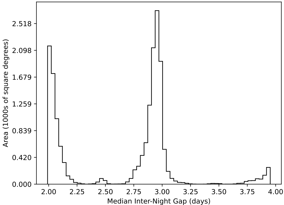
too_elab_r16_d2_gz_v3.4_10yrs WFD all bands: Median Inter-Night Gap
