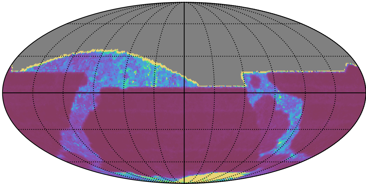
too_elab_r16_d2_gz_v3.4_10yrs All sky z band: Median Inter-Night Gap
