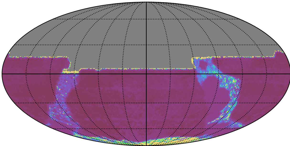
too_elab_r16_d2_gz_v3.4_10yrs All sky y band: Median Inter-Night Gap
