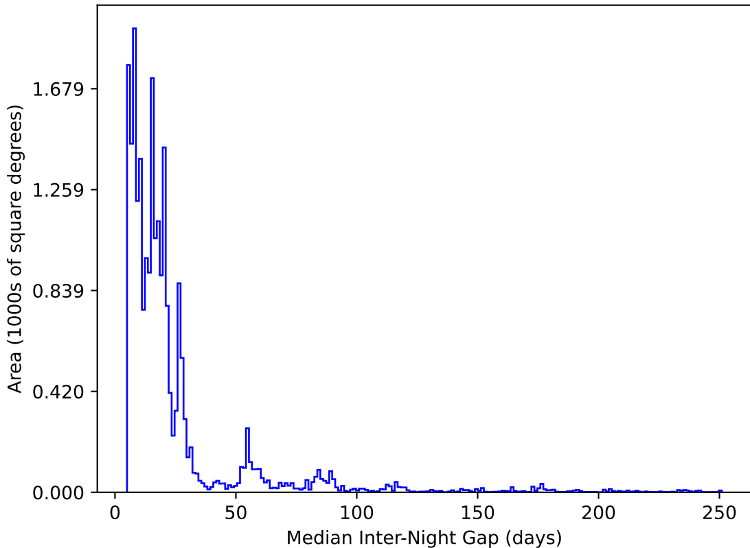
too_elab_r16_d2_gz_v3.4_10yrs All sky y band: Median Inter-Night Gap
