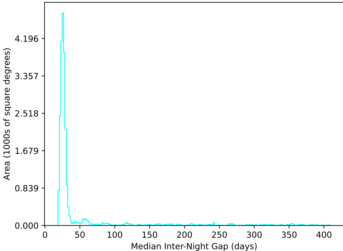
too_elab_r16_d2_gz_v3.4_10yrs All sky u band: Median Inter-Night Gap
