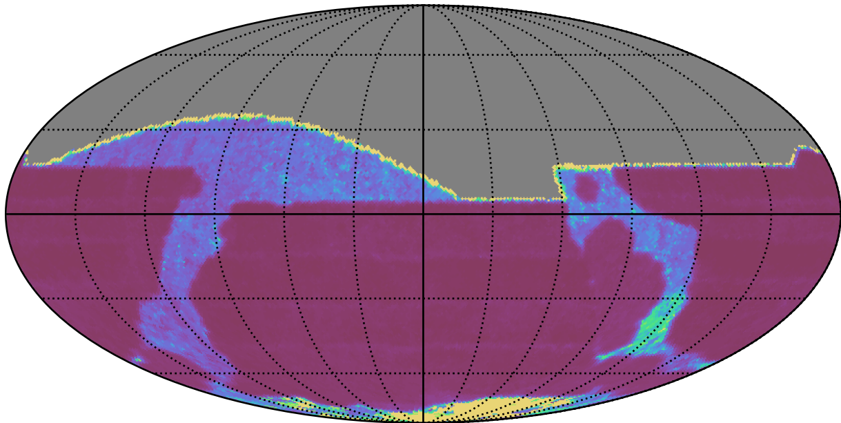
too_elab_r16_d2_gz_v3.4_10yrs All sky r band: Median Inter-Night Gap
