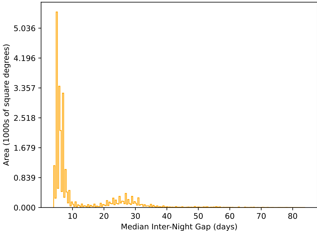
too_elab_r16_d2_gz_v3.4_10yrs All sky r band: Median Inter-Night Gap
