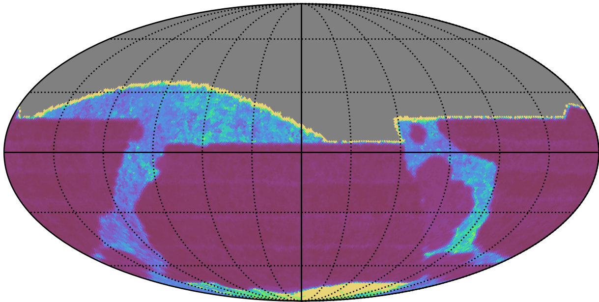
too_elab_r16_d2_gz_v3.4_10yrs All sky i band: Median Inter-Night Gap
