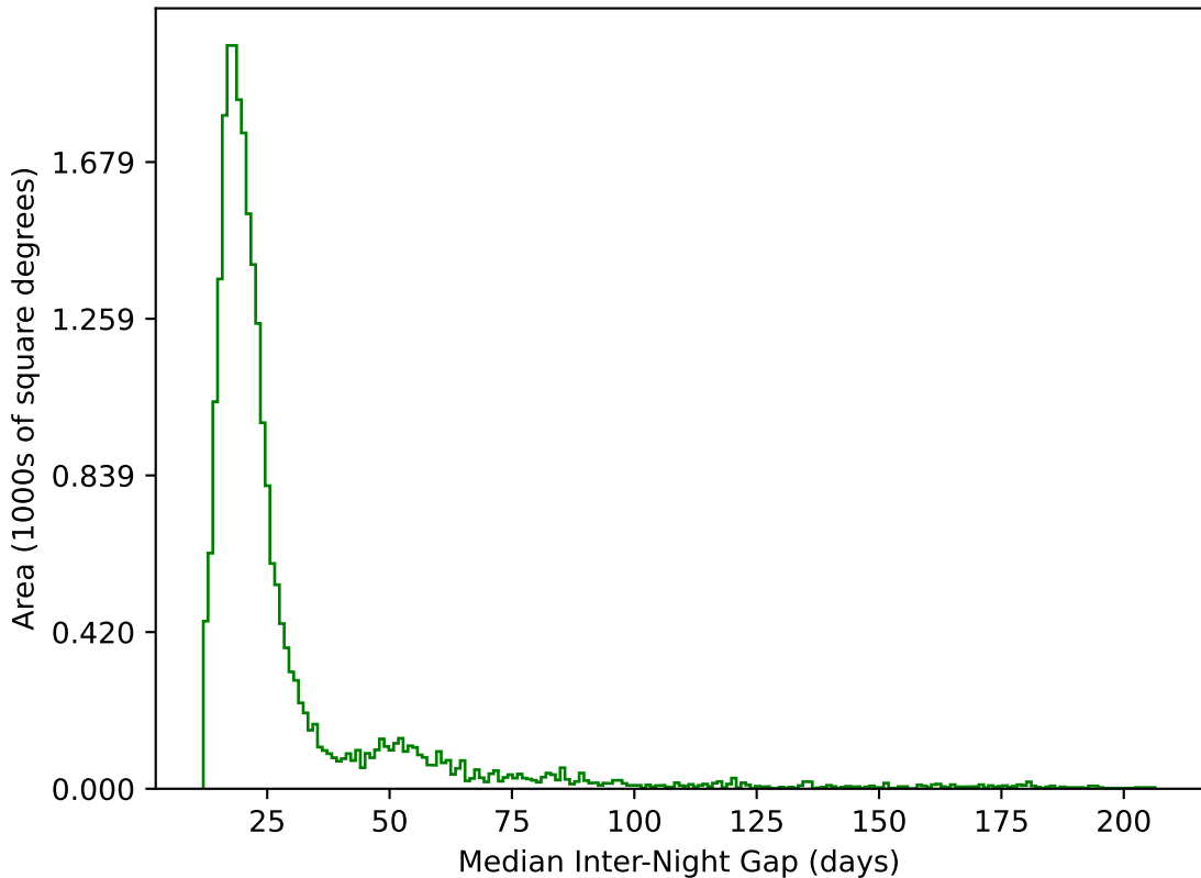
too_elab_r16_d2_gz_v3.4_10yrs All sky g band: Median Inter-Night Gap
