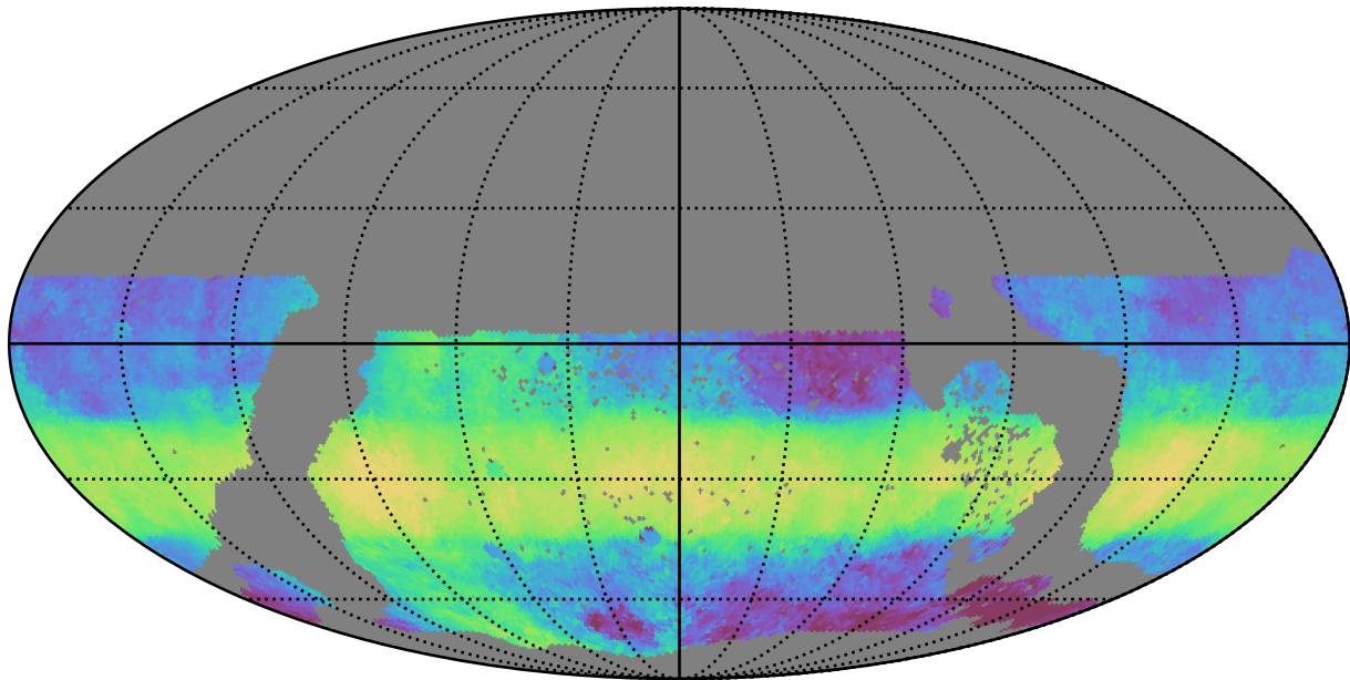
too_elab_r16_d2_gz_v3.4_10yrs WFD z band: Median HA
