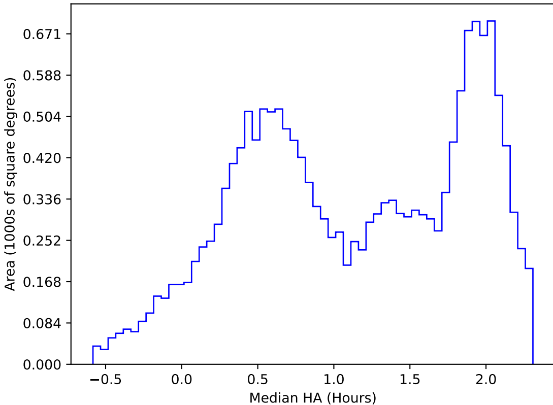
too_elab_r16_d2_gz_v3.4_10yrs WFD z band: Median HA
