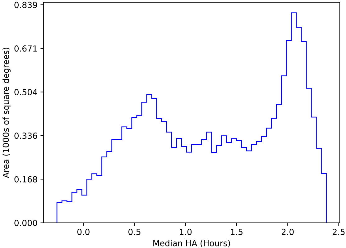
too_elab_r16_d2_gz_v3.4_10yrs WFD y band: Median HA
