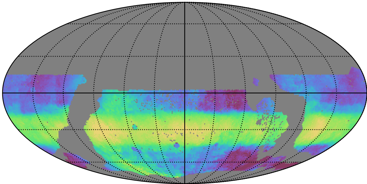
too_elab_r16_d2_gz_v3.4_10yrs WFD r band: Median HA
