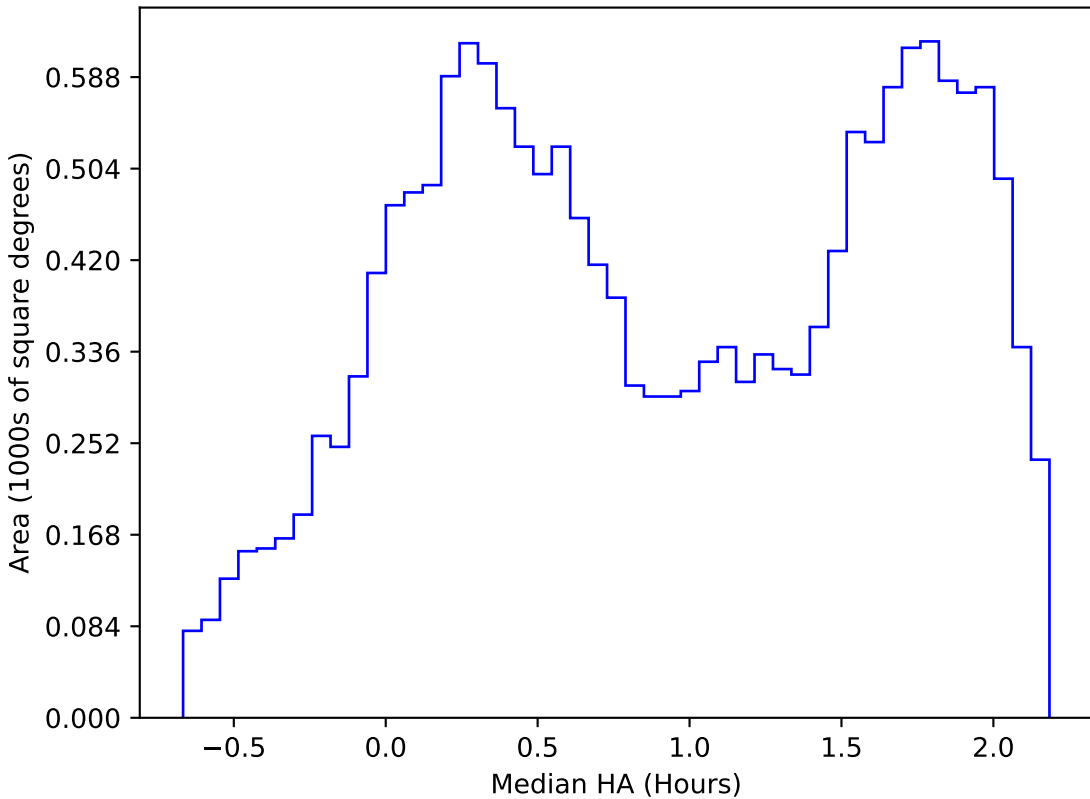
too_elab_r16_d2_gz_v3.4_10yrs WFD r band: Median HA
