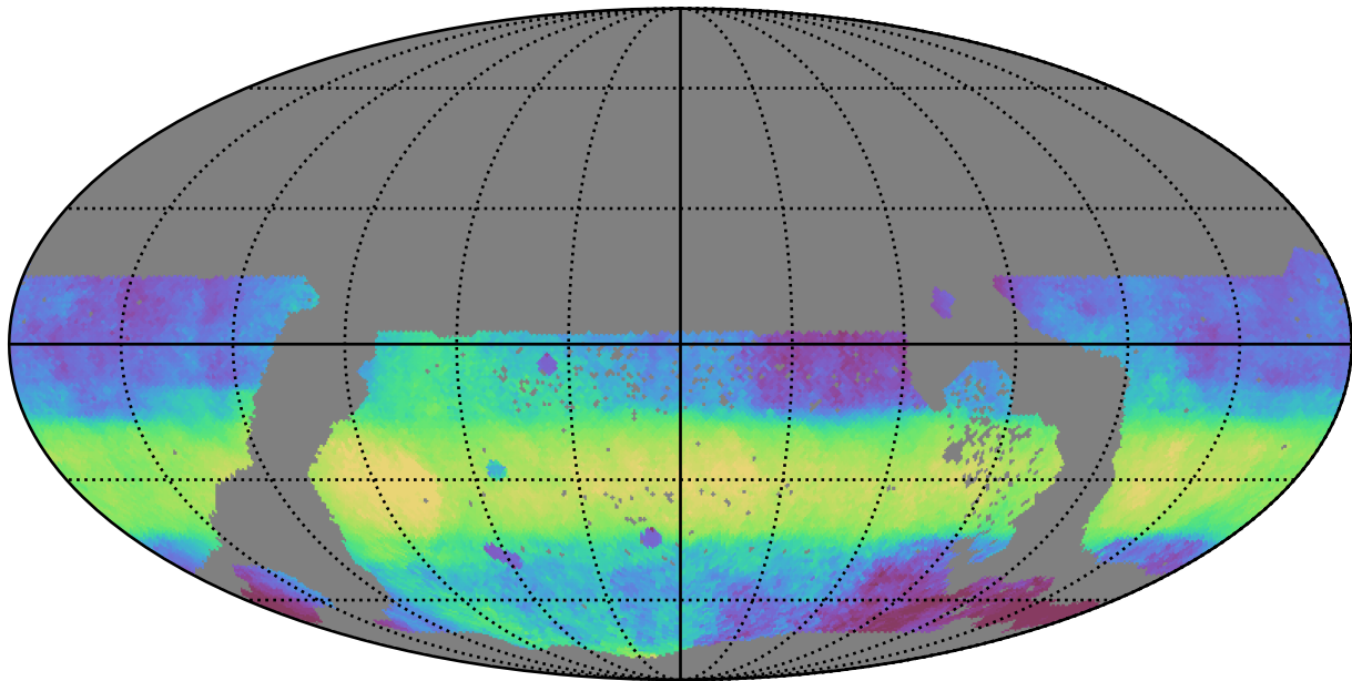
too_elab_r16_d2_gz_v3.4_10yrs WFD i band: Median HA
