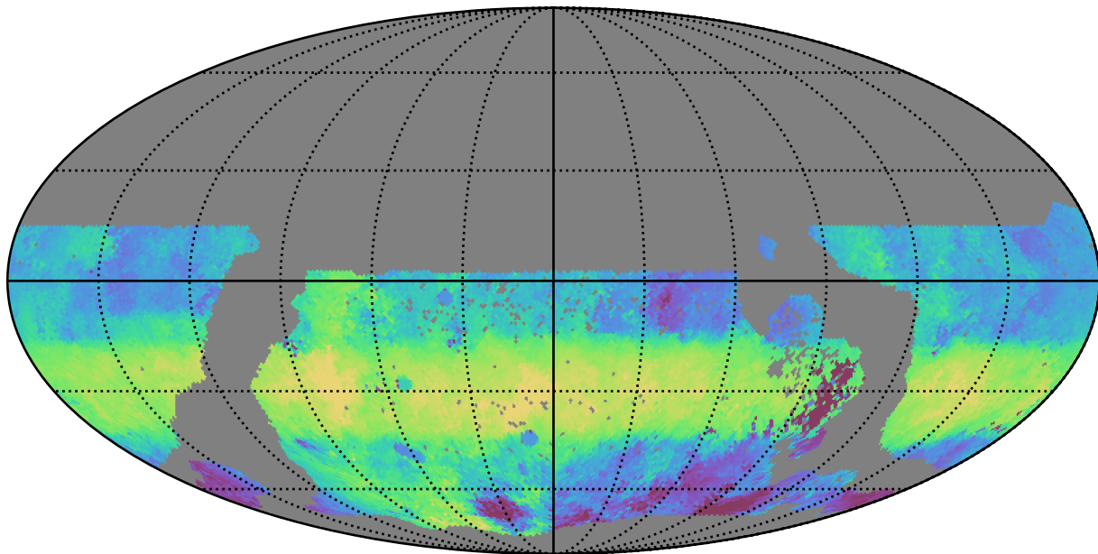
too_elab_r16_d2_gz_v3.4_10yrs WFD g band: Median HA
