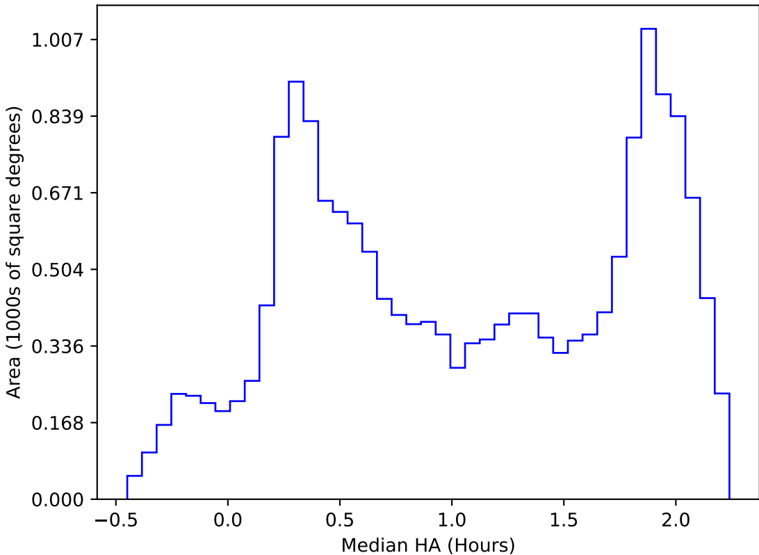
too_elab_r16_d2_gz_v3.4_10yrs WFD all bands: Median HA
