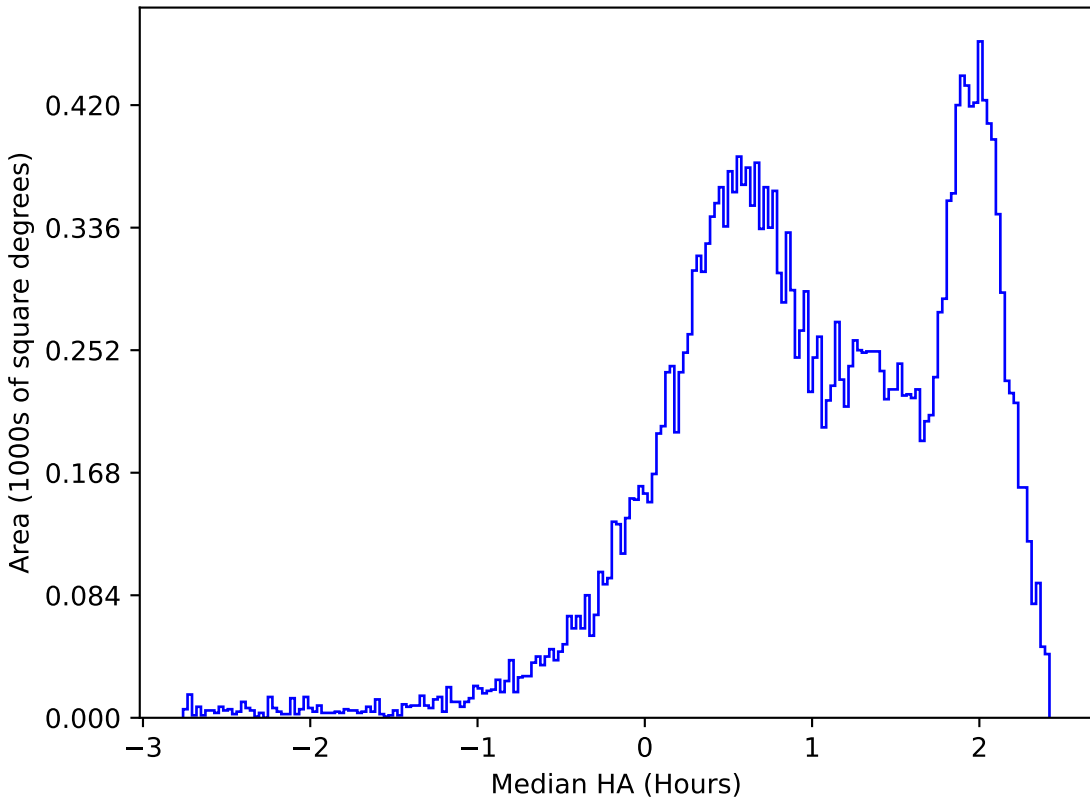
too_elab_r16_d2_gz_v3.4_10yrs All sky z band: Median HA
