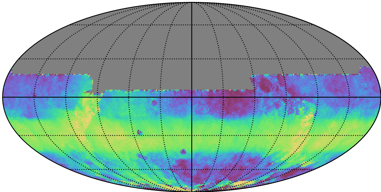
too_elab_r16_d2_gz_v3.4_10yrs All sky y band: Median HA
