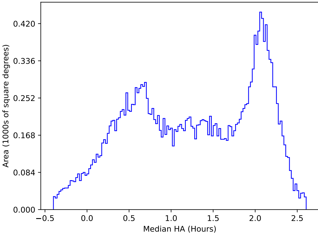
too_elab_r16_d2_gz_v3.4_10yrs All sky y band: Median HA
