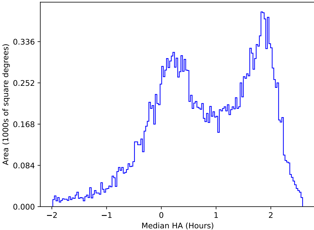
too_elab_r16_d2_gz_v3.4_10yrs All sky u band: Median HA
