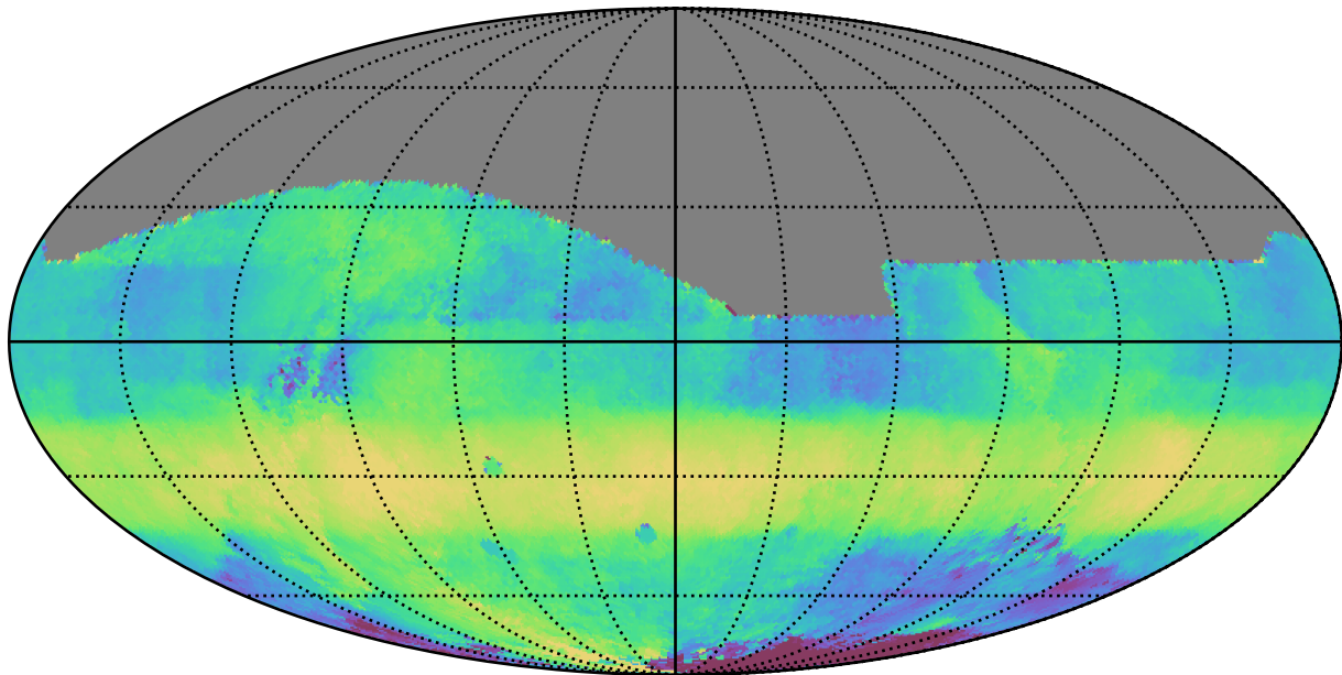
too_elab_r16_d2_gz_v3.4_10yrs All sky r band: Median HA
