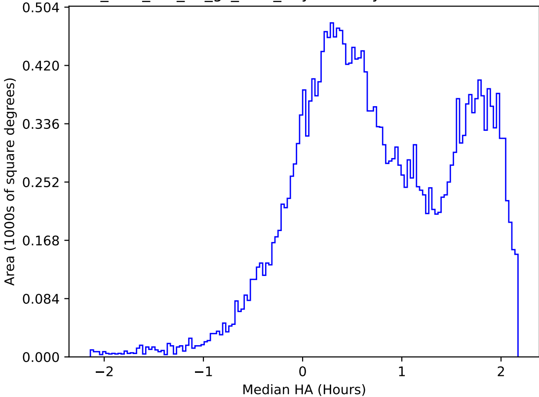
too_elab_r16_d2_gz_v3.4_10yrs All sky r band: Median HA
