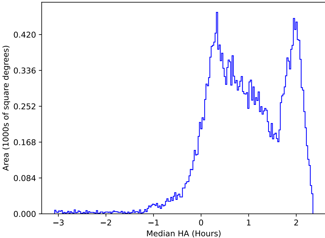
too_elab_r16_d2_gz_v3.4_10yrs All sky i band: Median HA
